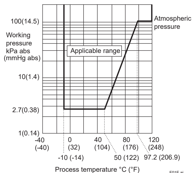
Figure 1. Working Pressure and Process Temperature [EJX530S Hygienic Silicone oil type(code: B)]
